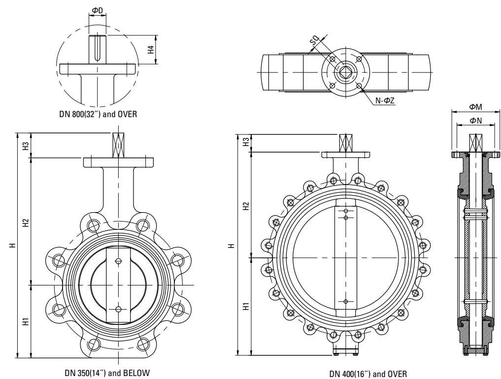
VALVE DIMENSIONS
