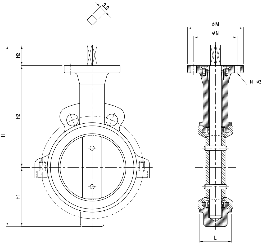
VALVE DIMENSIONS
